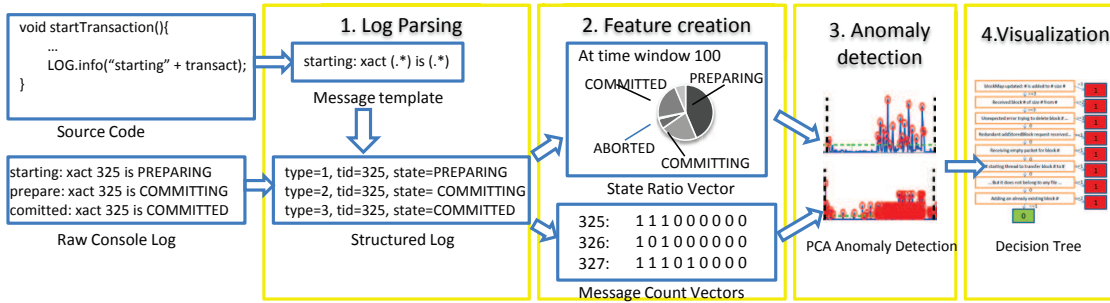
Figure 2. Overview of console log analysis work flow.
